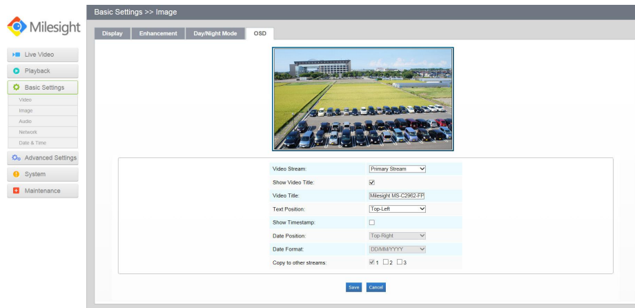
Figure 4-3-10 OSD
