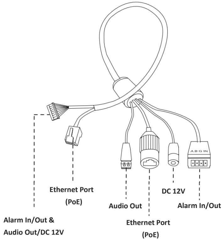
Figure 1-3-12 Pro Dome Network Camera multiple interface cable
