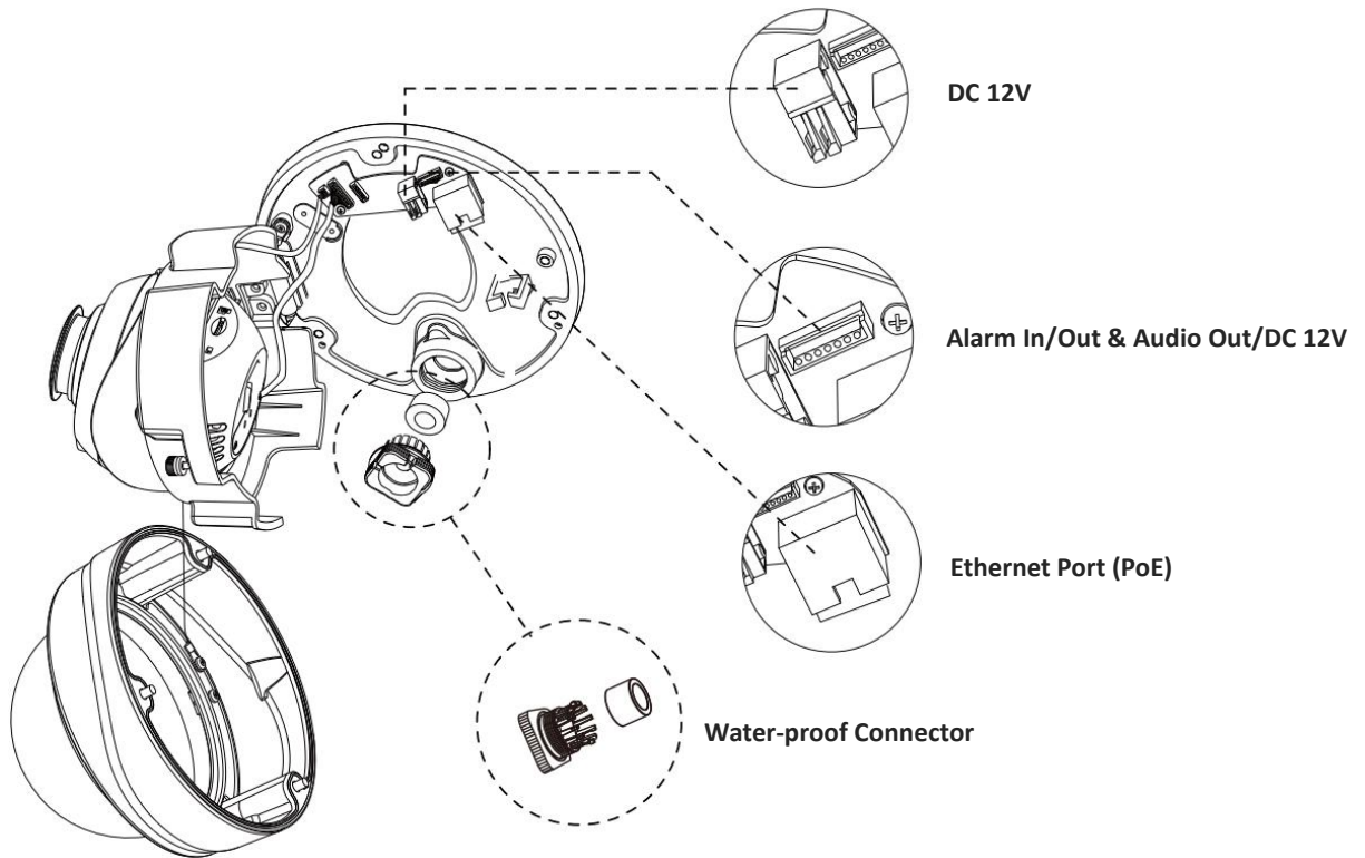
Figure 1-3-11 Pro Dome Network Camera multiple interface
