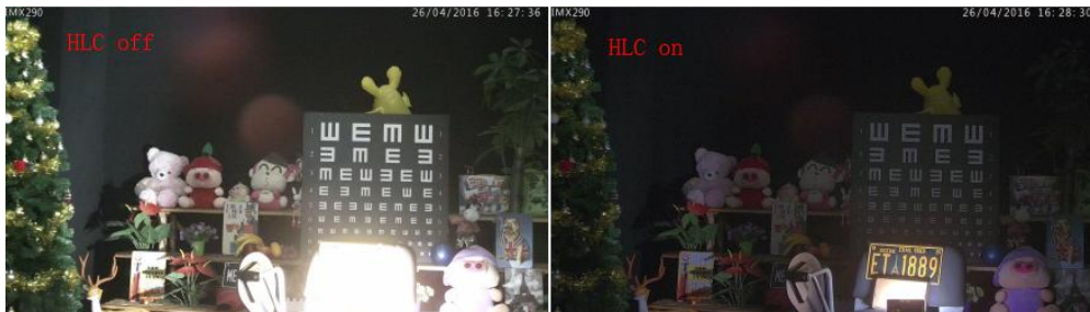
Figure 4-3-8 HLC Image
