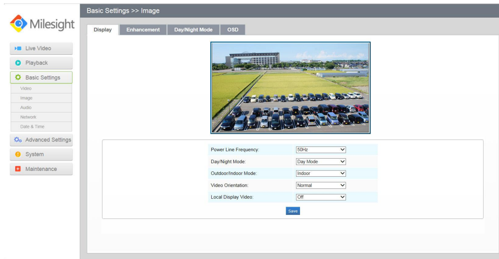
Figure 4-3-4 Display
