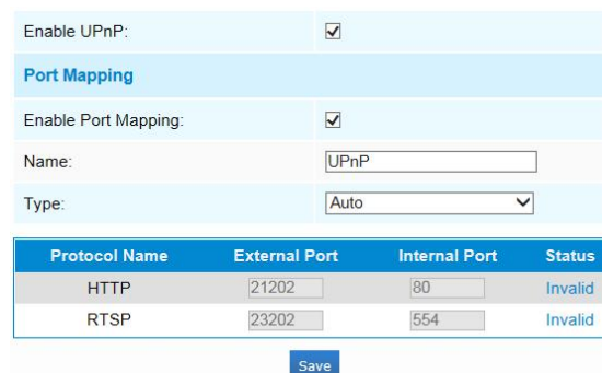
Figure 4-4-3 UPnP Settings
