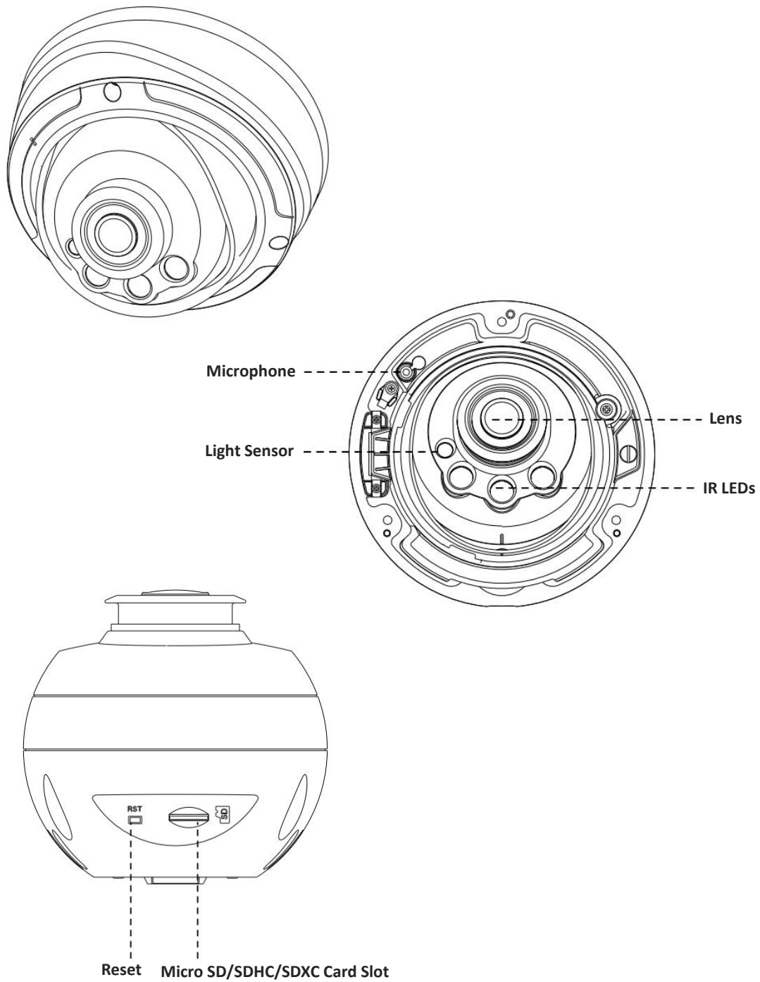
Figure 1-3-10 Pro Dome Network Camera
