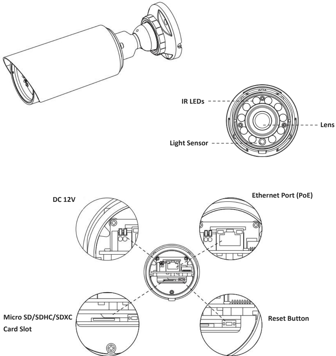
Figure 1-3-6 Remote Focus&Zoom Mini Bullet Network Camera
