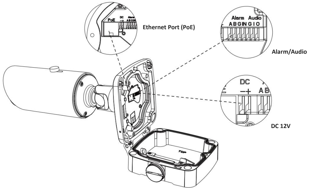
Figure 1-3-8 Pro Bullet Network Camera (Version A)
