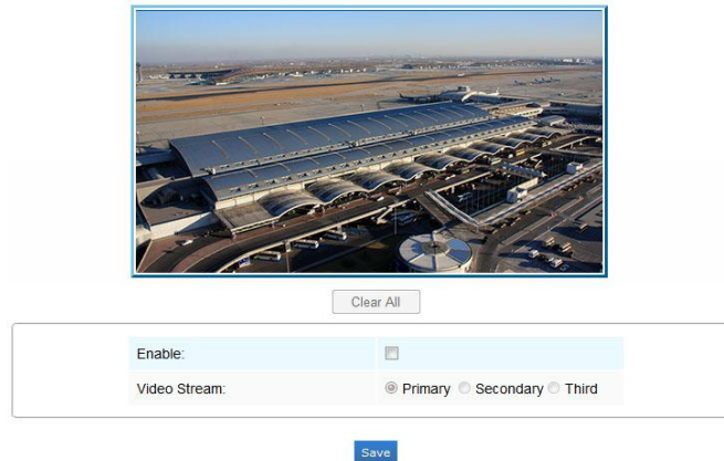
Figure 4-4-2 ROI Settings
