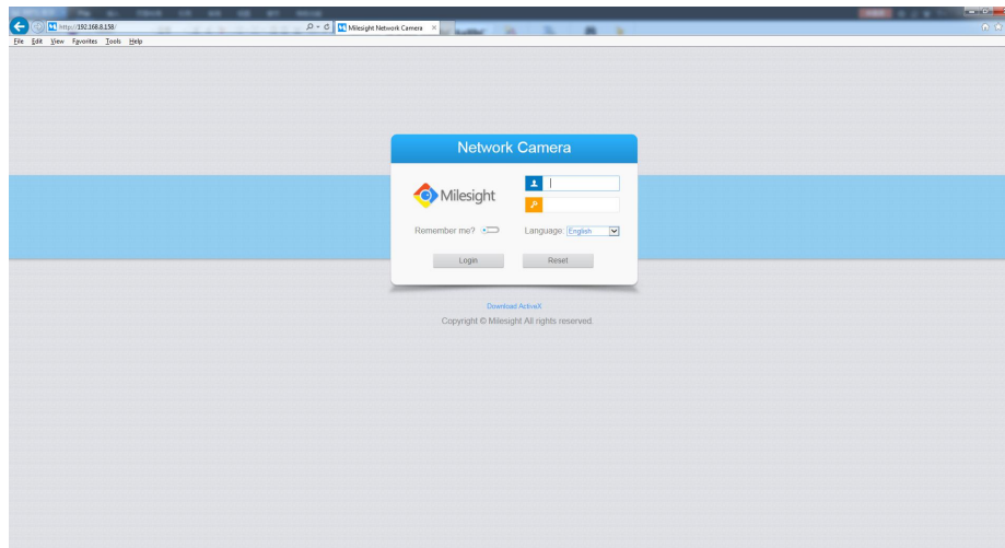
Figure 3-1-7 Login interface
