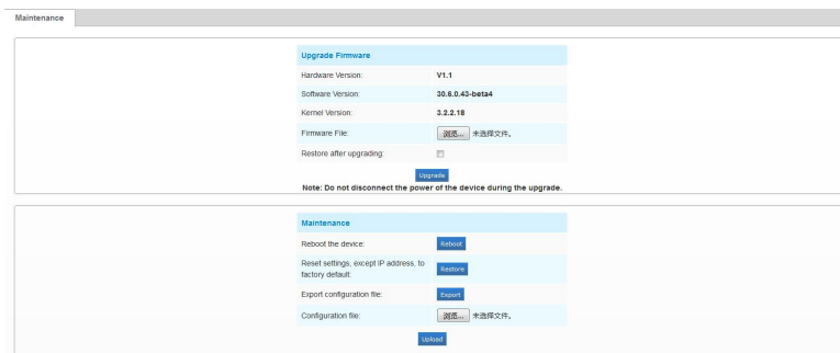
Figure 4-5-2 Maintenance
