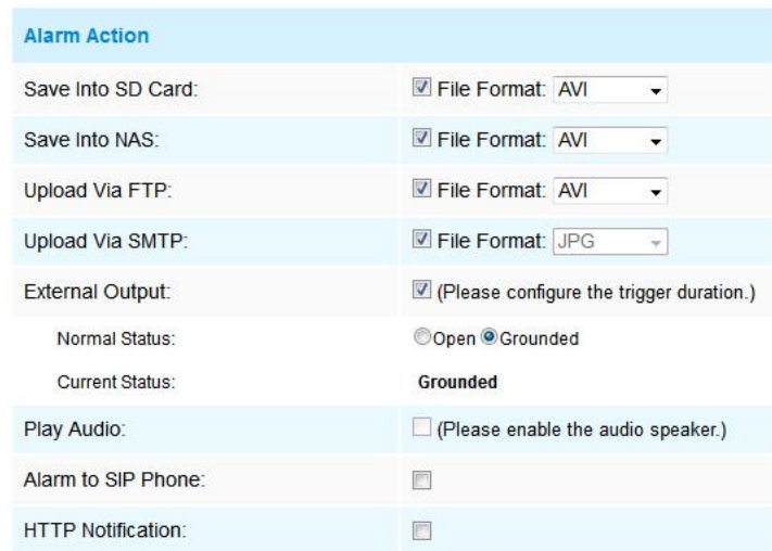
Figure 4-4-12 Alarm Action
