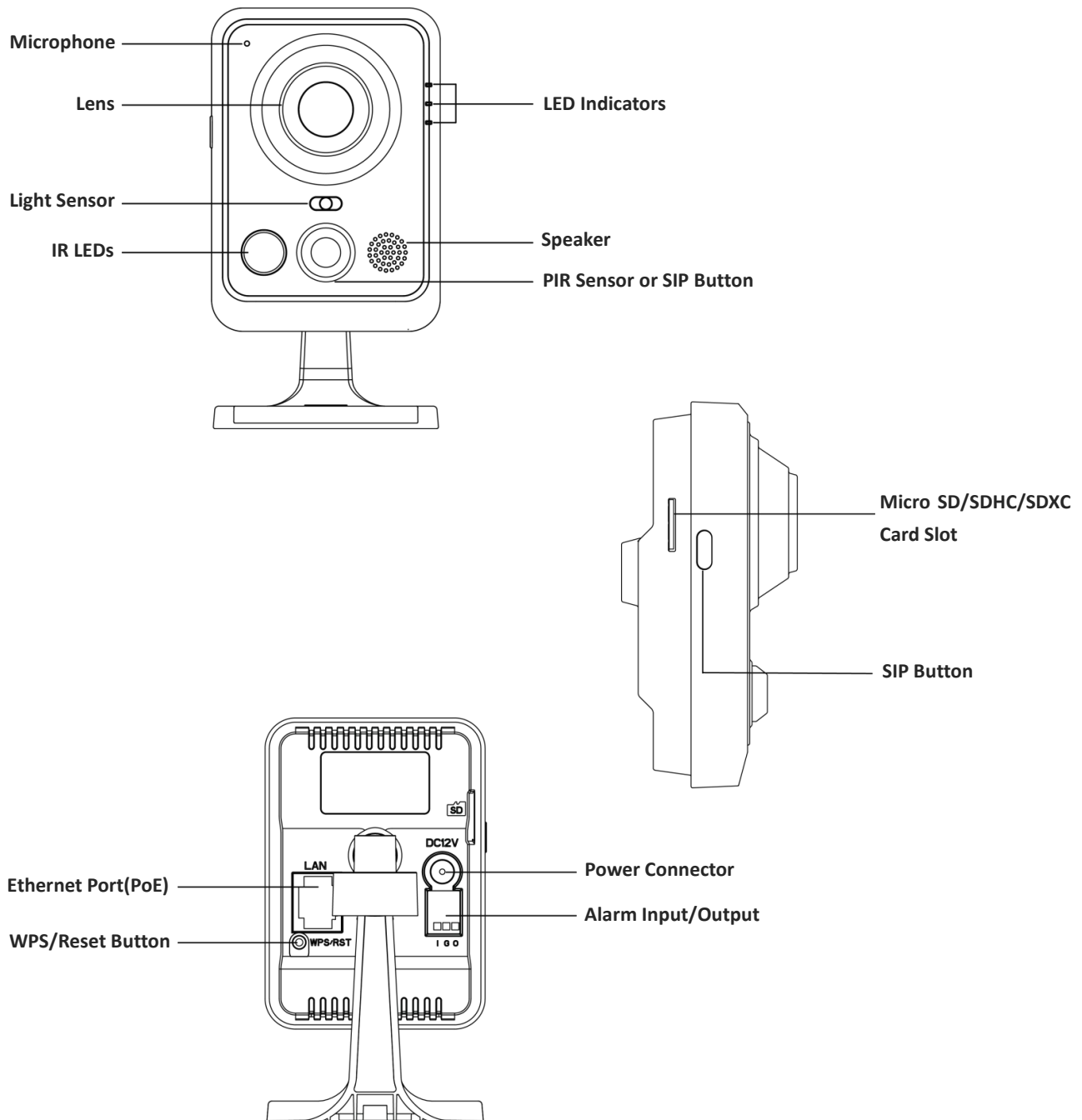
Figure 1-3-4 Wi-Fi Mini Cube Network Camera
