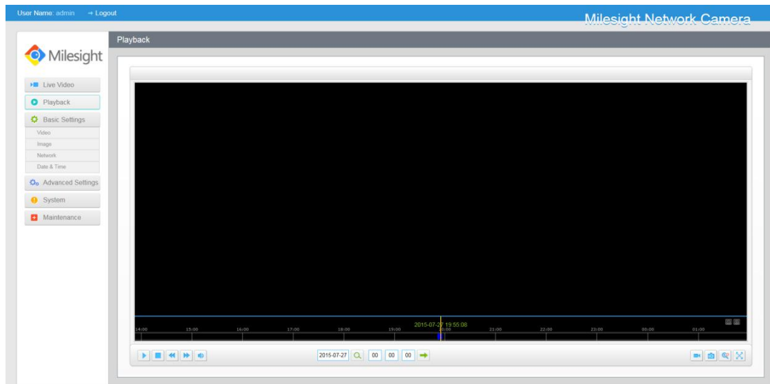
Figure 4-2-1 Playback interface
